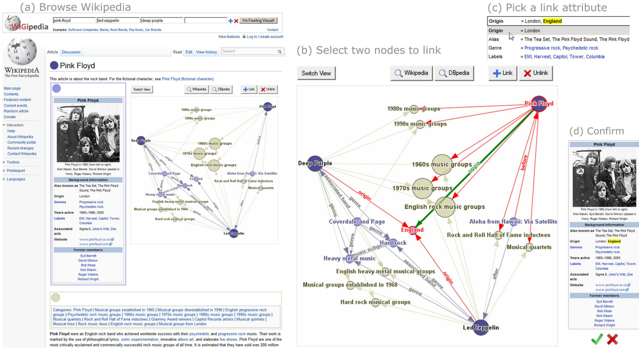
Fig. 2. WiGipedia components: (a) shows a wiki article for “Pink Floyd” with an embedded contextual graph of semantically linked articles. In (b) dark blue nodes represent the starting point for the graph generation. In this case three English bands: “Pink Floyd”, “Led Zeppelin”, and “Deep Purple”. The remainder of the graph represents commonalities between them: light blue nodes are other wiki articles (i.e. “England”) and tan nodes are Wikipedia categories (i.e. “1980s music groups”). A user created edge is highlighted in green. (c) shows the drop-down menu with a list of suggested labels for the new edge. In this example “Pink Floyd” and “England” are linked by “Origin”. (d) shows a confirmation step that occurs before the new update is propagated to Wikipedia.
